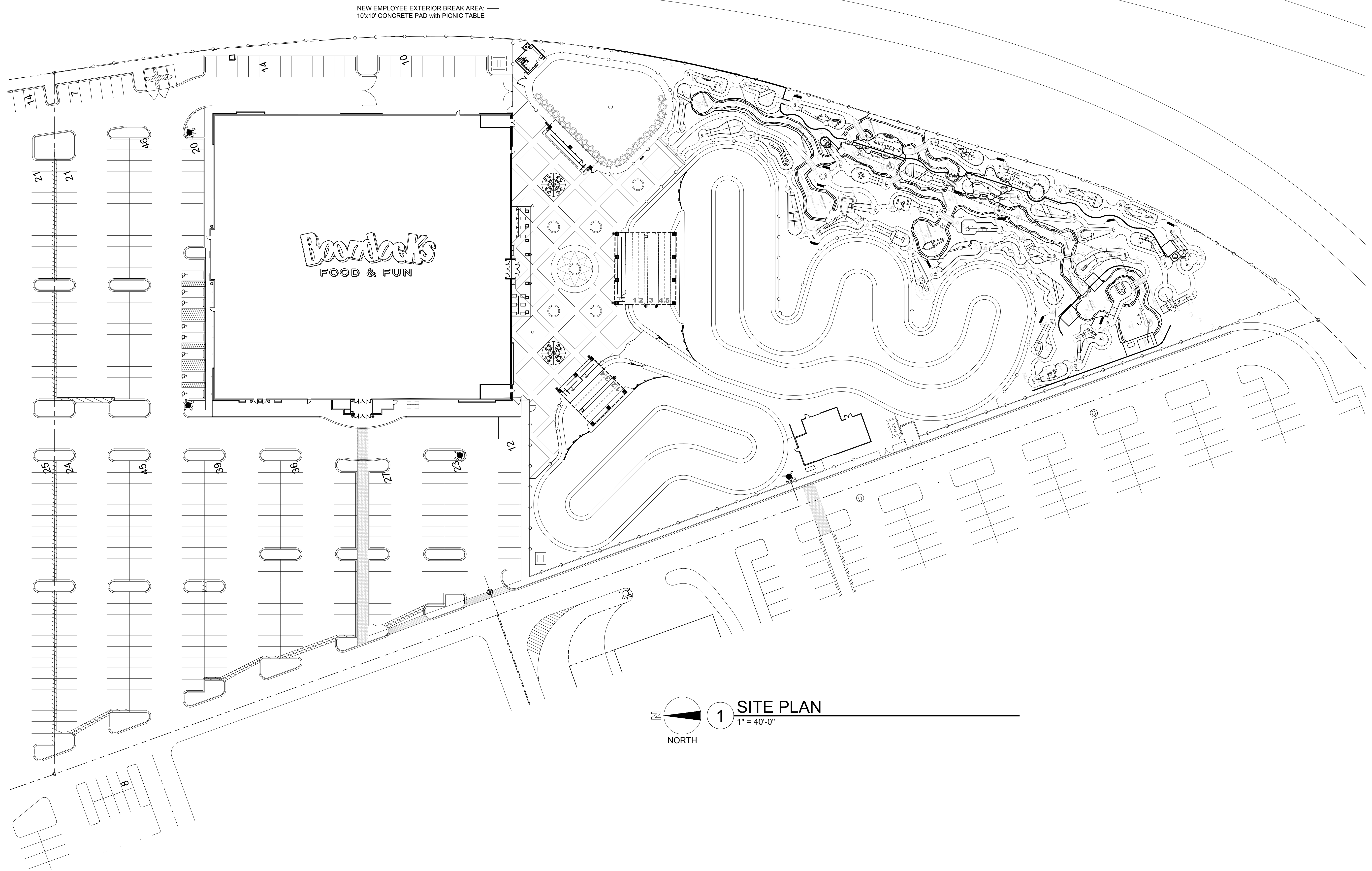
0 20' 40' 80' 1" = 40'-0"
