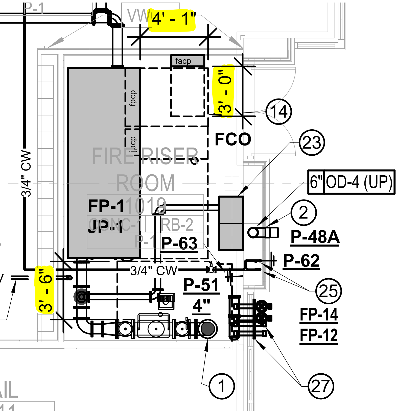
FIRE PUMP RISER ROOM NOT TO SCALE
