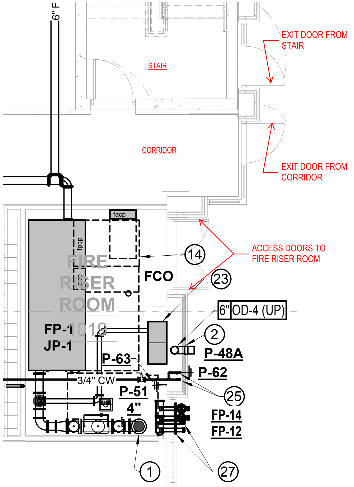
FIRE PUMP RISER ROOM NOT TO SCALE
