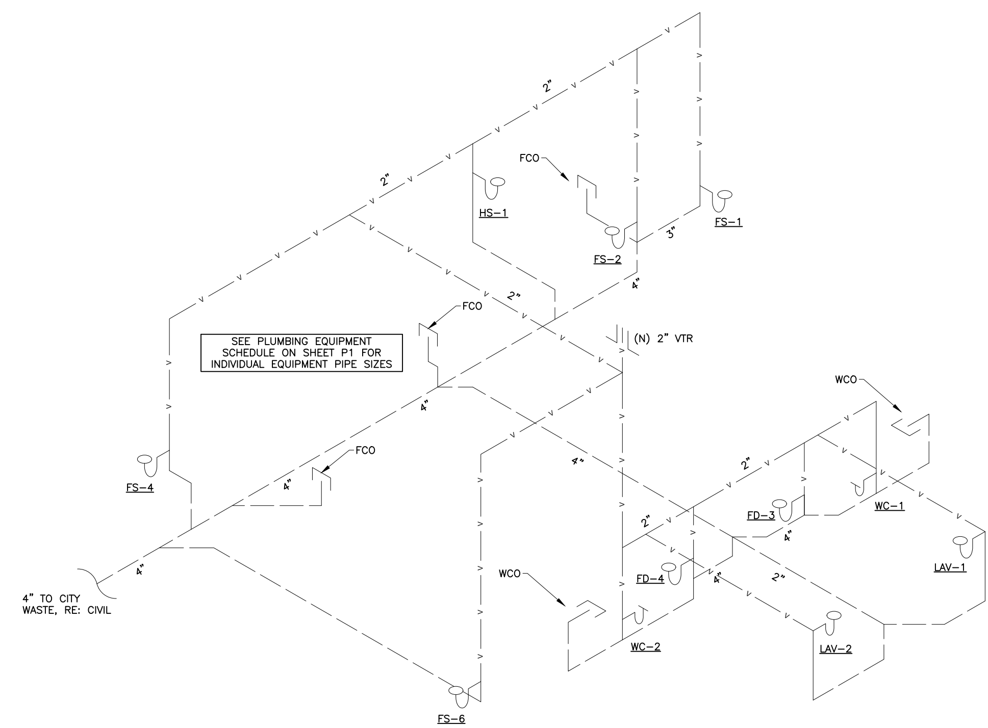
WASTE & VENT PIPING ISOMETRIC NOT TO SCALE
