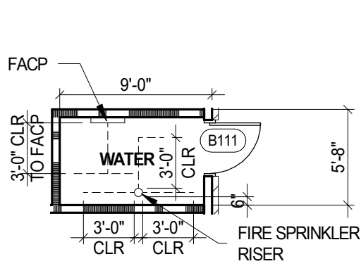
A BLDG A 1/8" = 1'-0"
