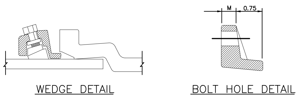
MECHANICAL JOINT RESTRAINT
