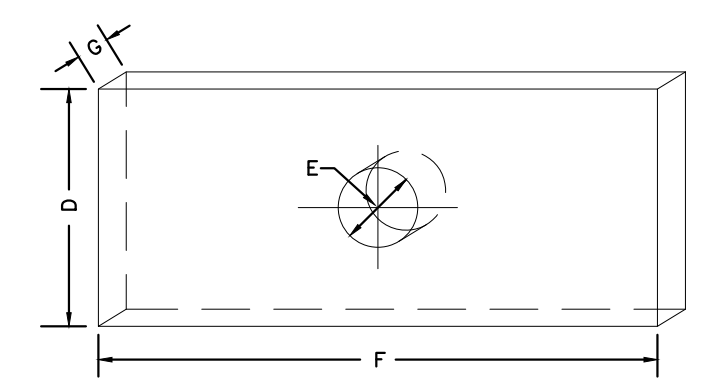
WASHER DETAIL
