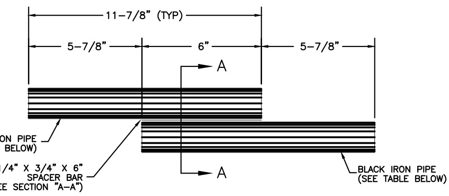
TIE ROD COUPLING DETAIL
