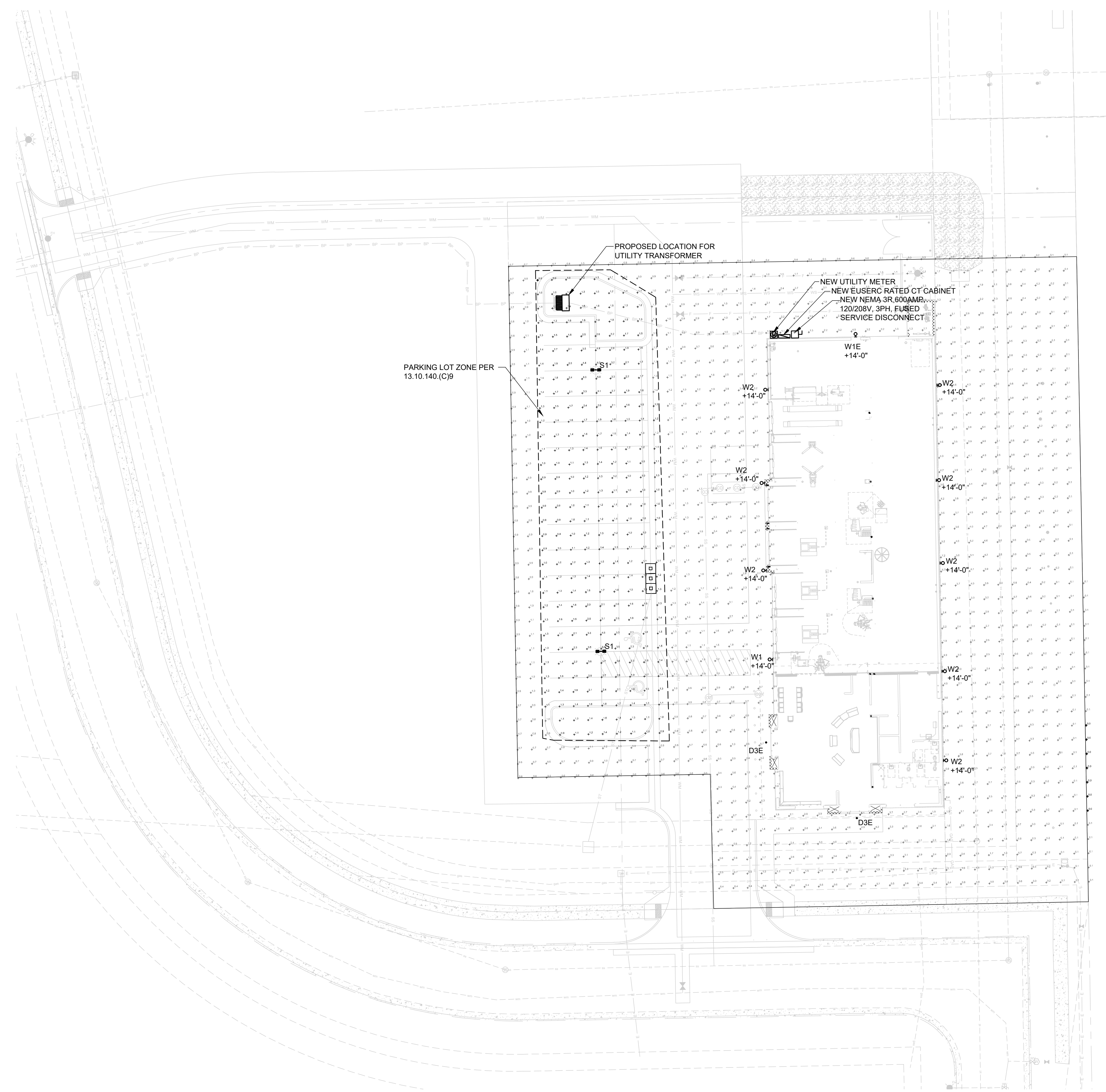
1 SITE PHOTOMETRIC PLAN NORTH REF. SCALE: 1" = 20'-0"
