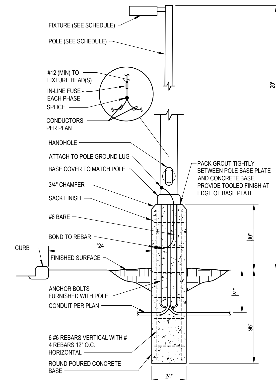
2 POLE DETAIL
