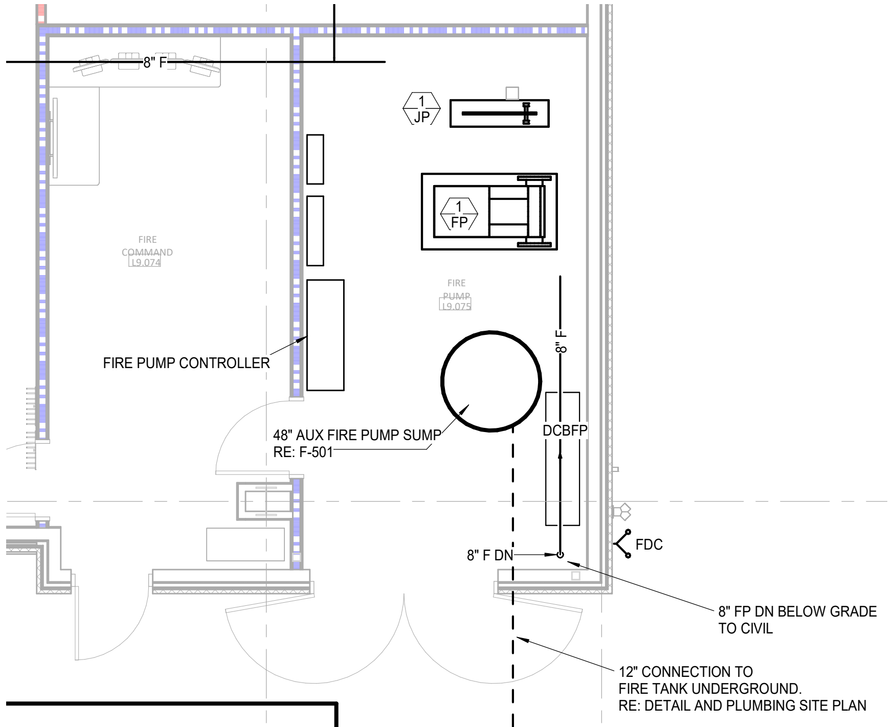
ENLARGED MECHANICAL PLAN - FIRE COMMAND AND PUMP ROOM
