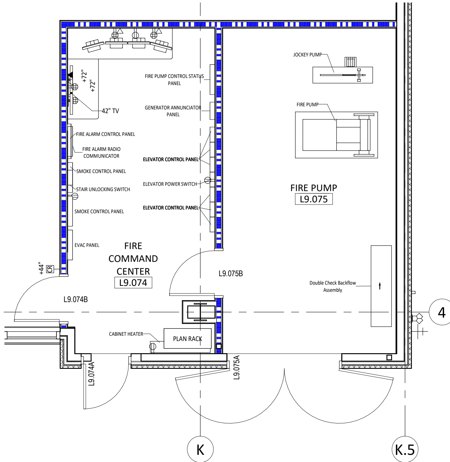
ENLARGED PLAN - FIRE COMMAND AND PUMP ROOM
