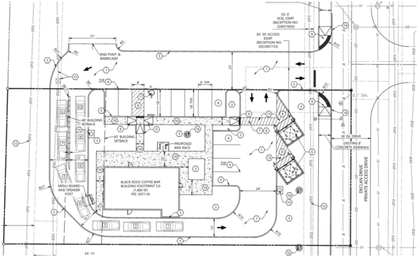
Figure 2 – Site Plan
