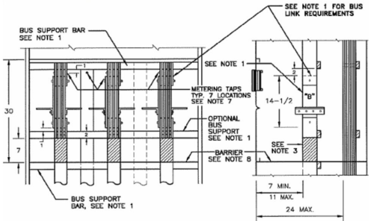
FRONT VIEW
