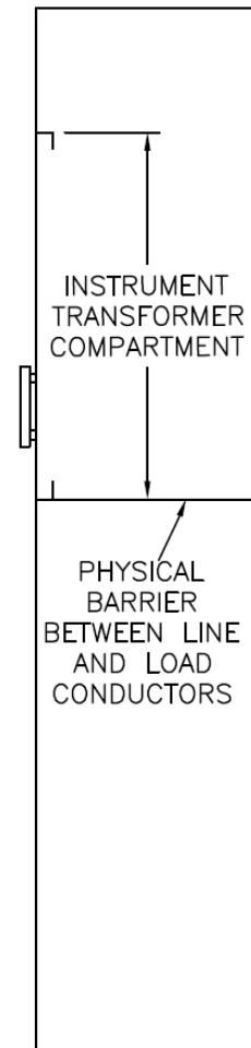
SIDE VIEW
