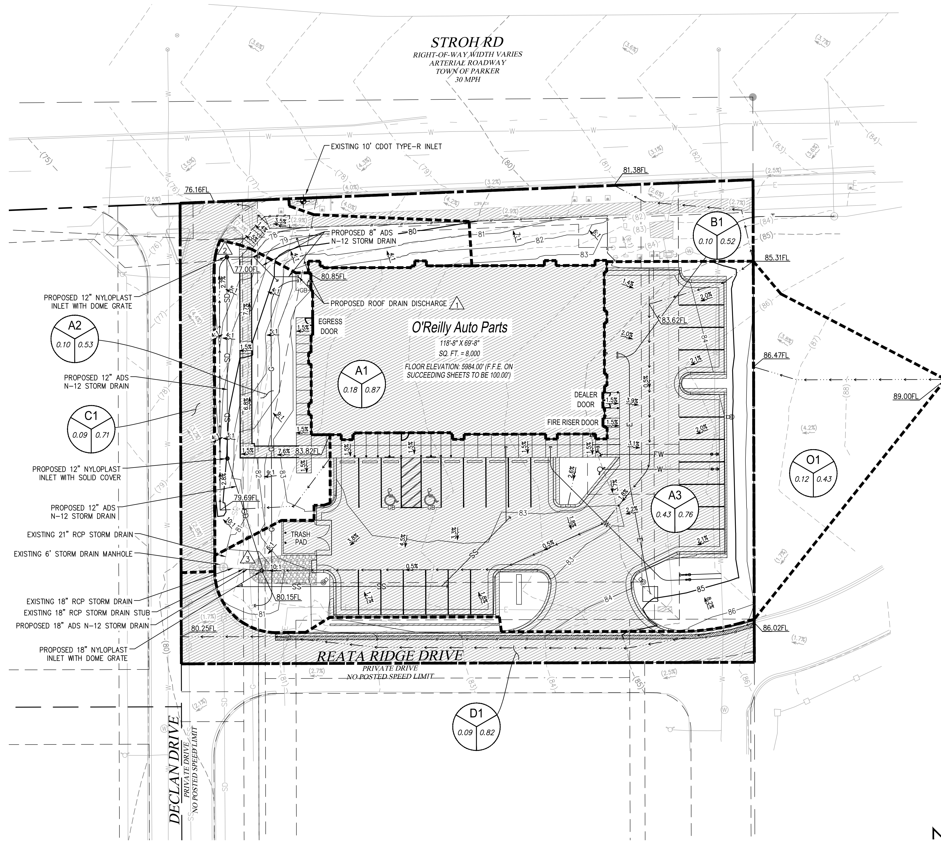
1 DEVELOPED DRAINAGE PLAN DR2 SCALE: 1" = 20'-0"
