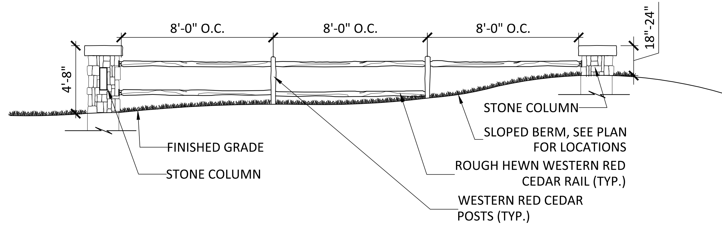
A SPLIT RAIL FENCE ELEVATION
