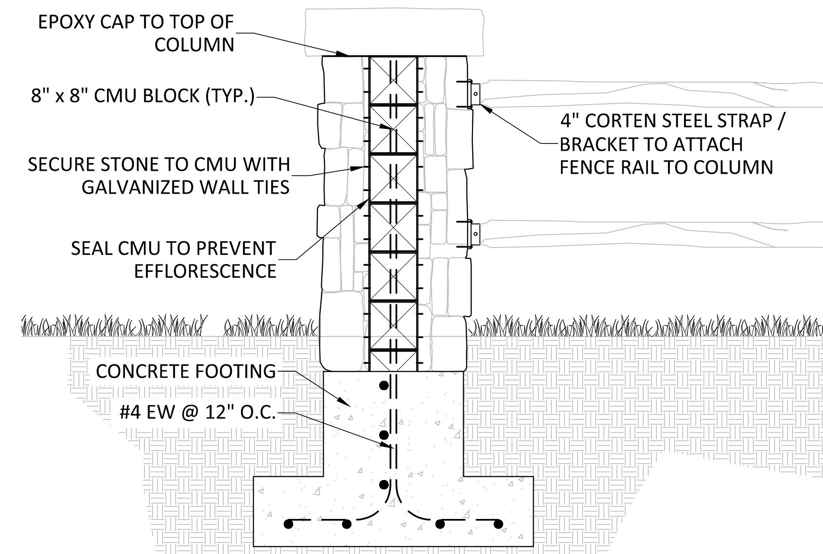
C STONE COLUMN STRUCTURAL DETAIL
