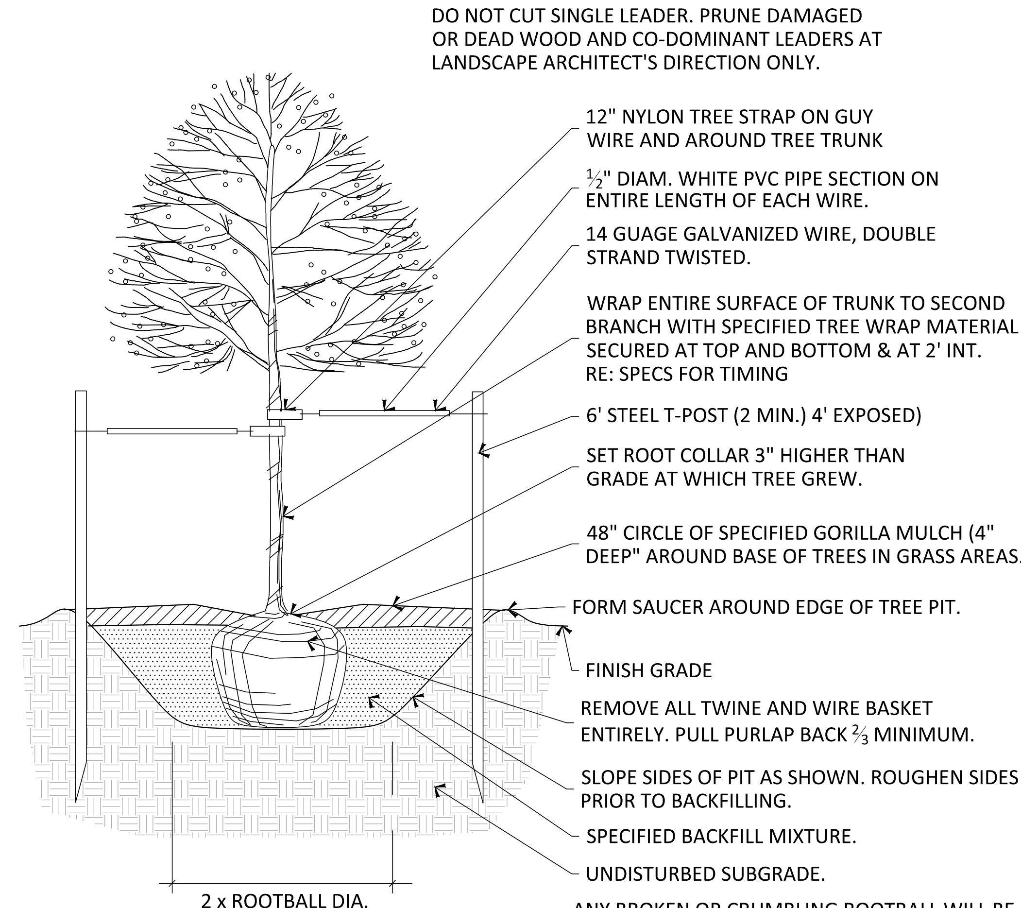
F DECIDUOUS TREE PLANTING DETAIL
