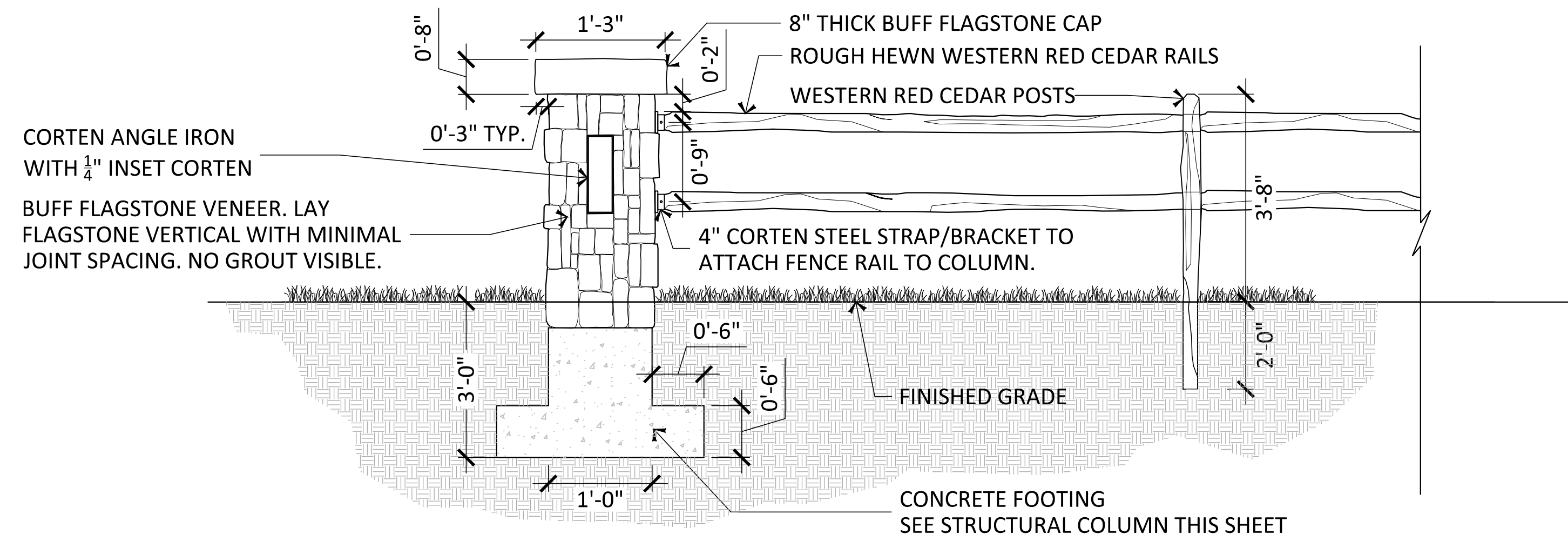
B STONE COLUMN DETAIL
