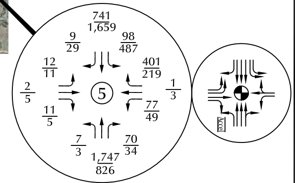
Figure 3 Existing Traffic, Lane Geometry and Traffic Control Trails at Crowfoot (LSC #160711)
