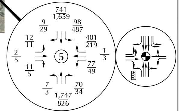
Figure 3 Existing Traffic, Lane Geometry and Traffic Control
