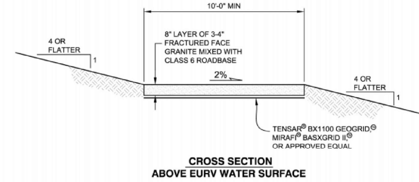
MAINTENANCE ROAD DETAILS N.T.S.
