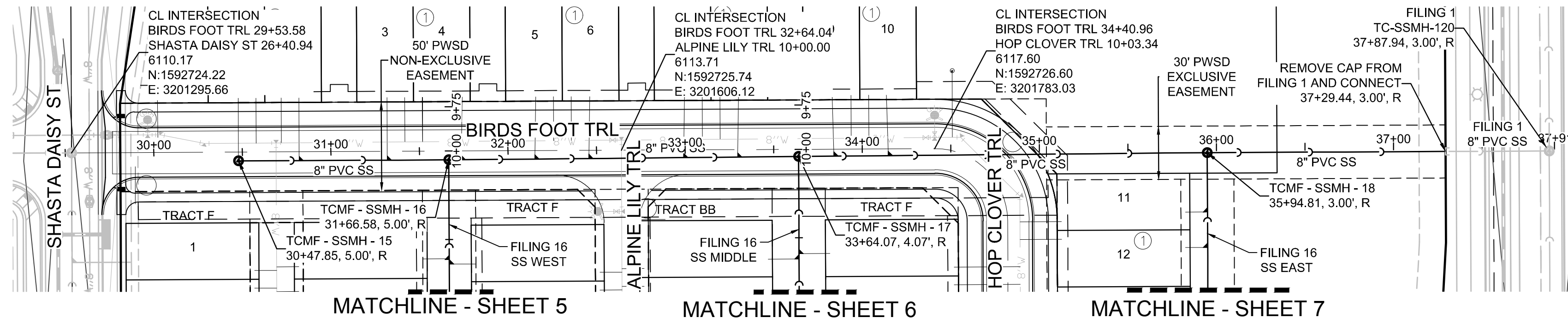
PLAN: BIRDS FOOT TRL STA: 29+00.00 TO 38+00.00 HORIZONTAL SCALE: 1" = 50'
