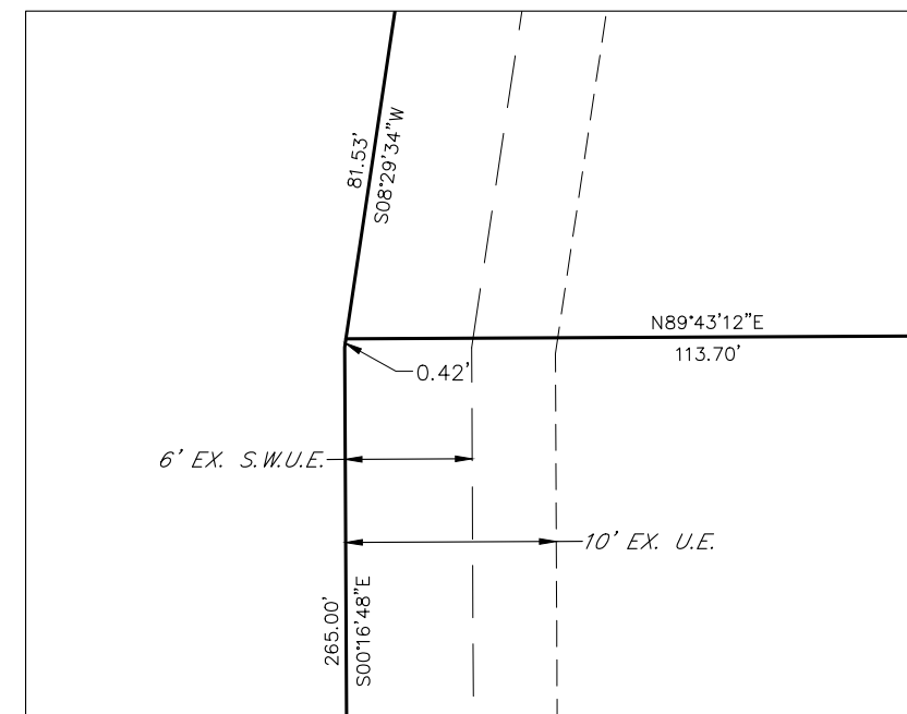
DETAIL B
