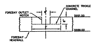
FOREBAY OUTLET NOTCH
