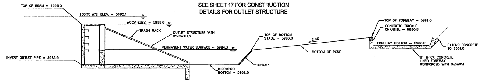
POND A: CROSS SECTION NOT TO SCALE
