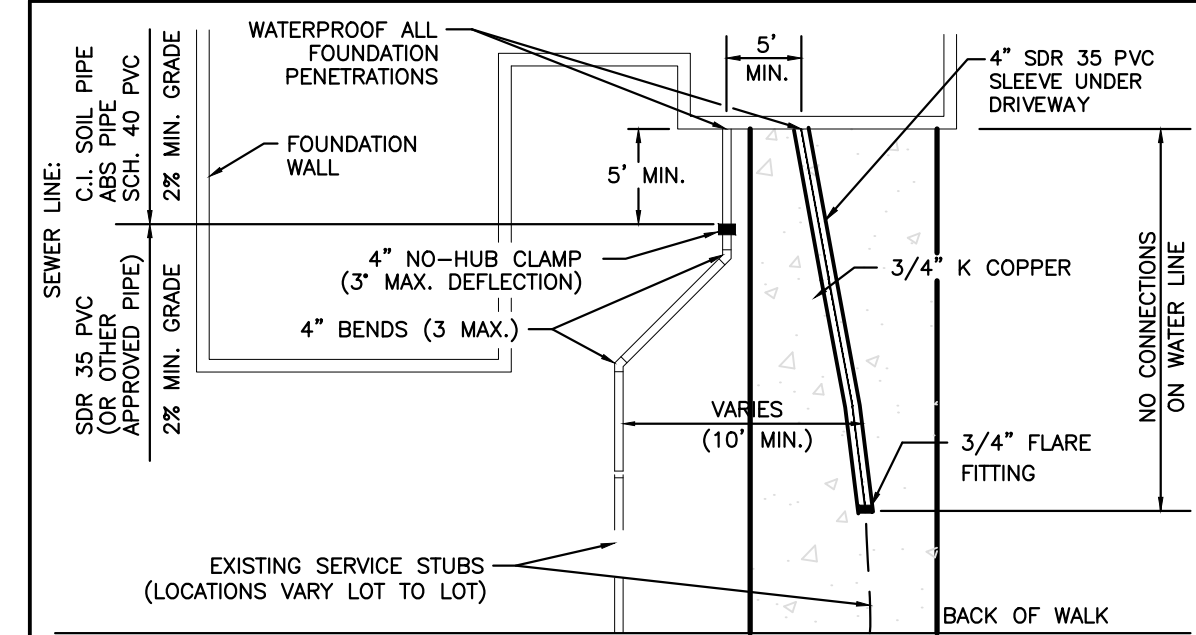
TYPICAL SERVICES PLAN VIEW NTS
