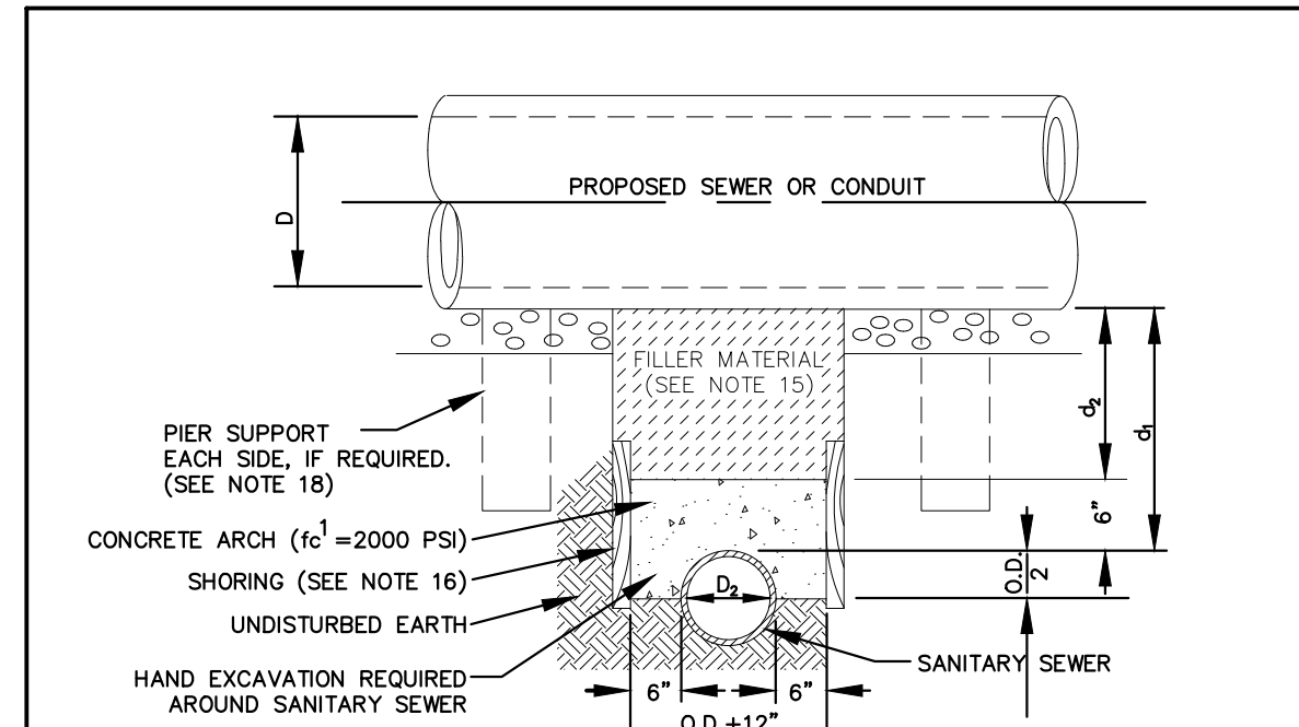
TYPE I CONCRETE ENCASEMENT FOR SANITARY SEWERS
