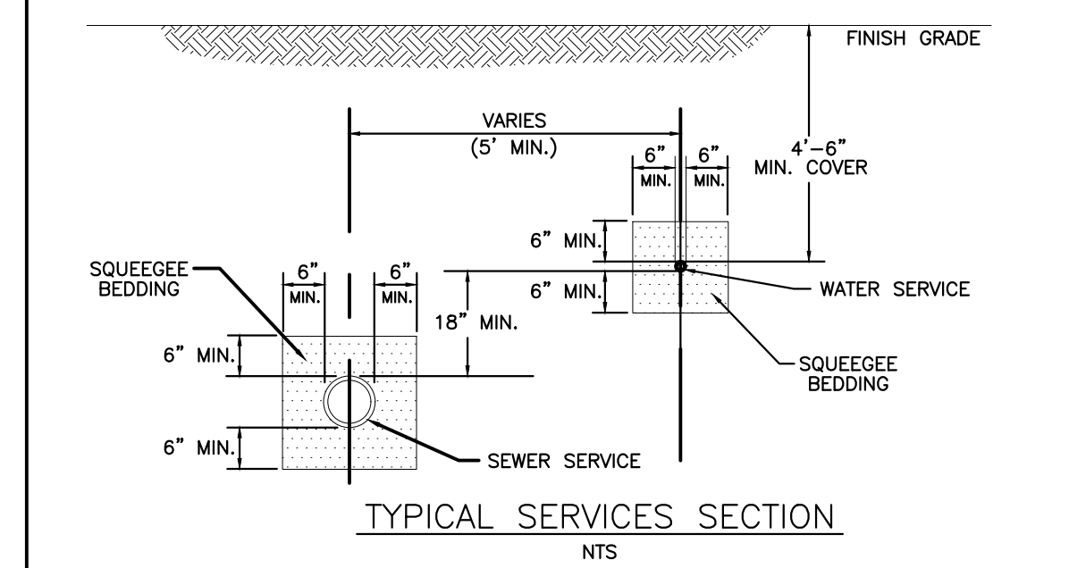
TYPICAL SERVICES SECTION NTS
