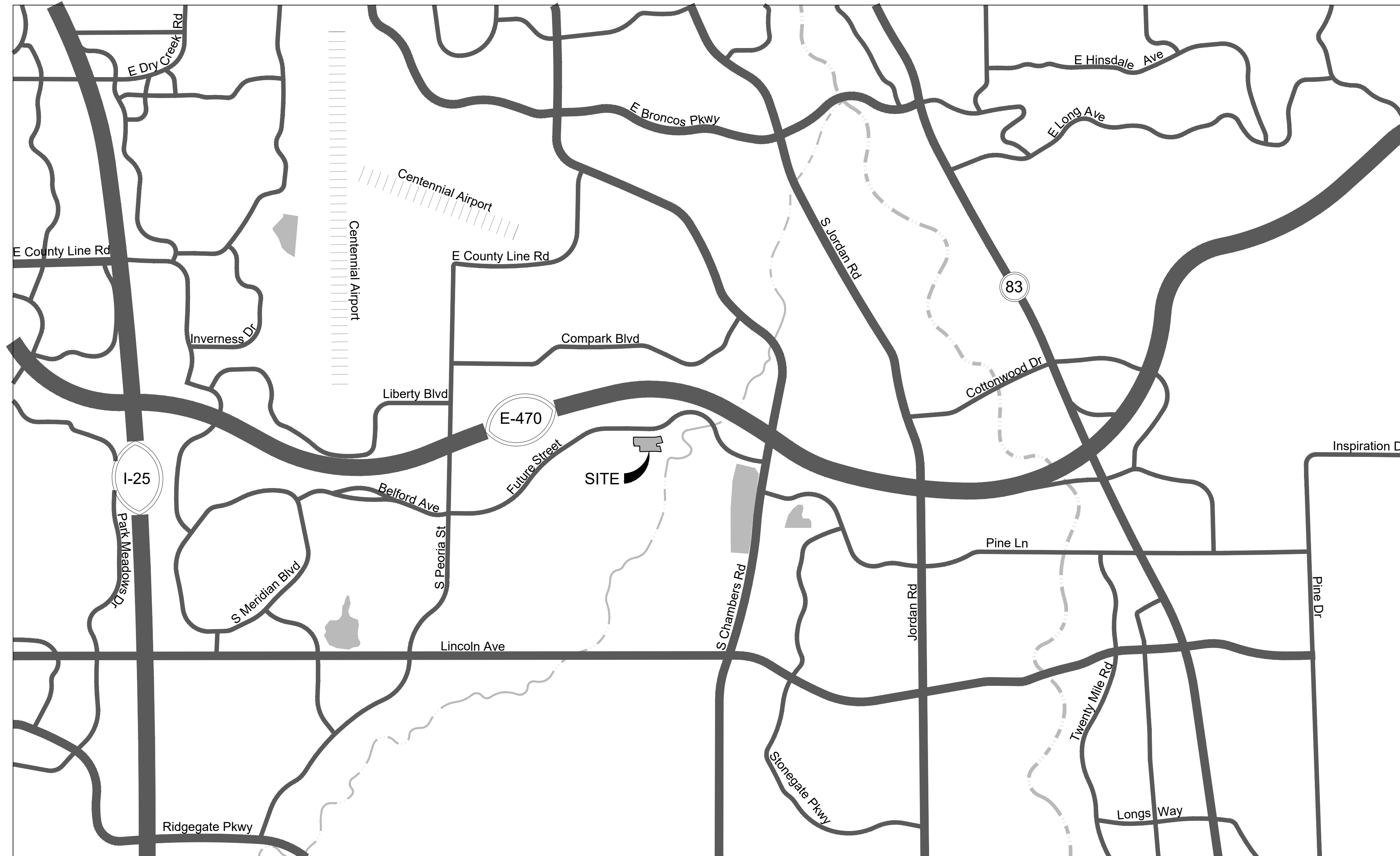
1 VICINITY MAP
