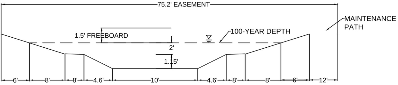
CHANNEL SECTION A-A NO TO SCALE
