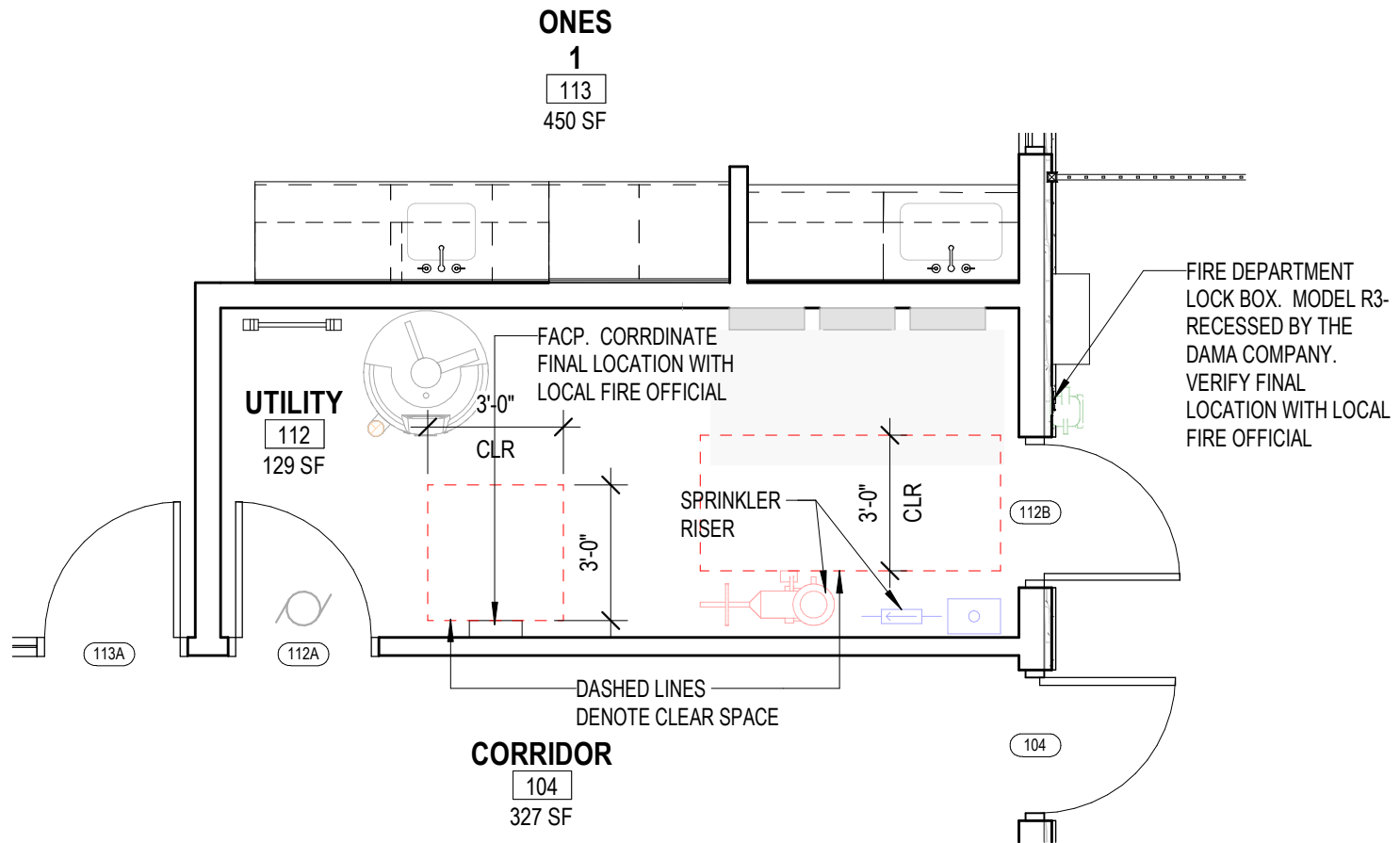
1 ENLARGED FIRE SPRINKLER PLAN 1/4" = 1'-0"
